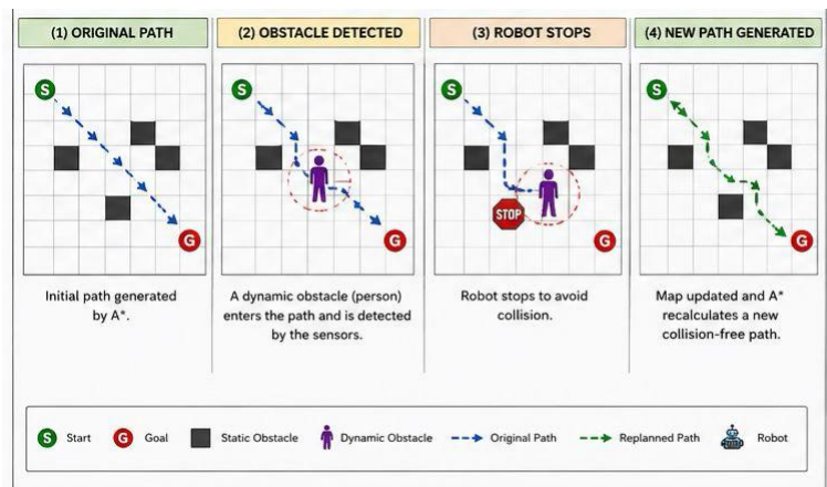
Fig 3 :Dynamic Avoidance
